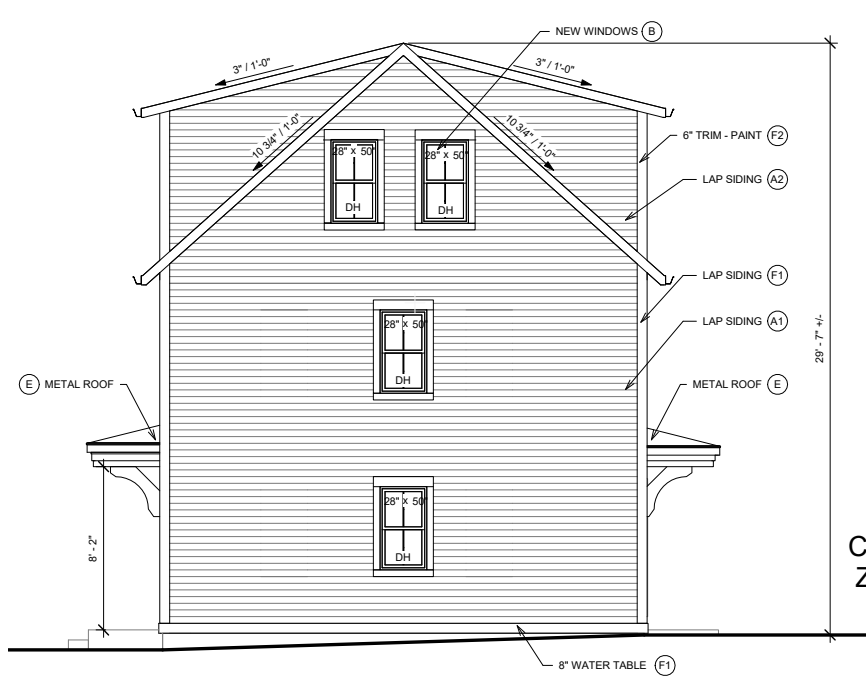
C4 NORTH ELEVATION 1/4" = 1'-0"
