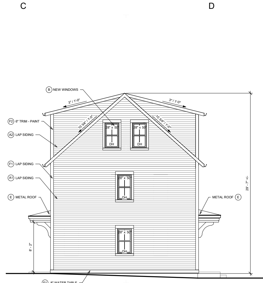
C2 SOUTH ELEVATION 1/4" = 1'-0"
